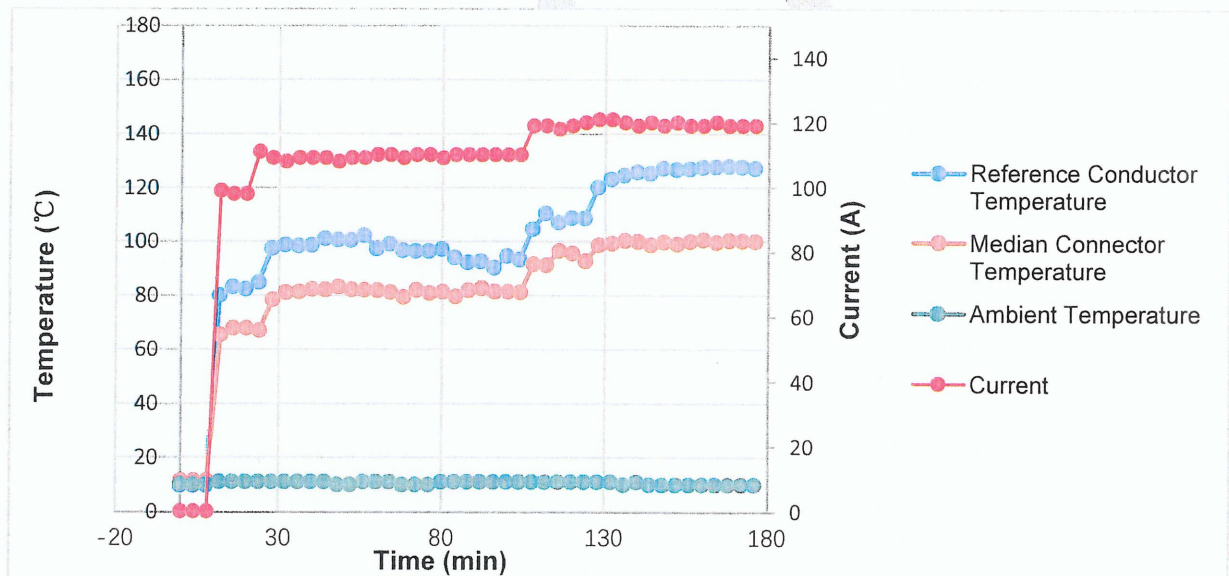
Figure 1 1st heat cycle temperature curve
