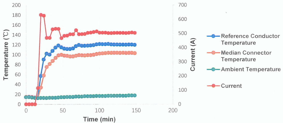
Figure 1 1st heat cycle temperature curve
