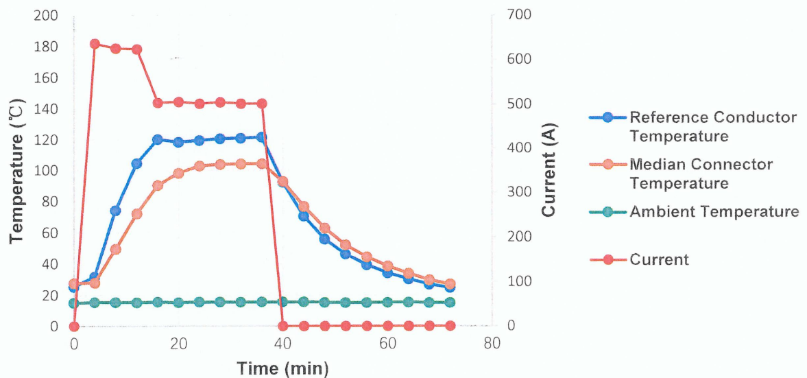
Figure 2 2nd heat cycle temperature curve
